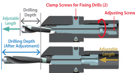
Fig.3 Adjustment of Drilling Depth
