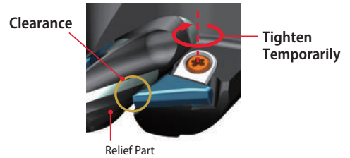
Fig.2 Install Inserts
