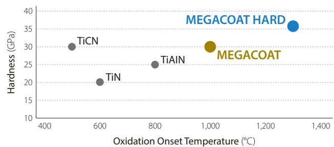
Coating Properties (Comparison with our conventional grade)
